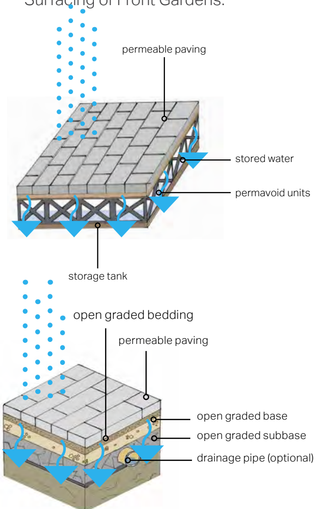
Figure 58: Diagrams illustrating the functioning of a soak away
